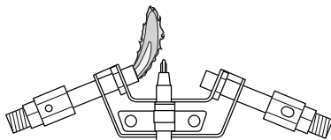
Figure 23 - Incorrect Pilot Flame Pattern
