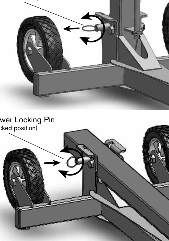
Tower Locking Pin (unlocked position)
