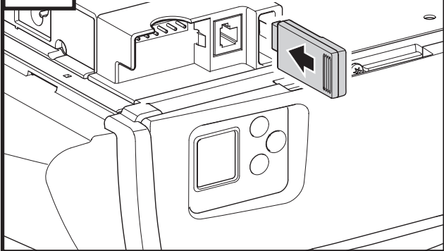
Fig. 37 Modular Antenna Installation or Replacement
