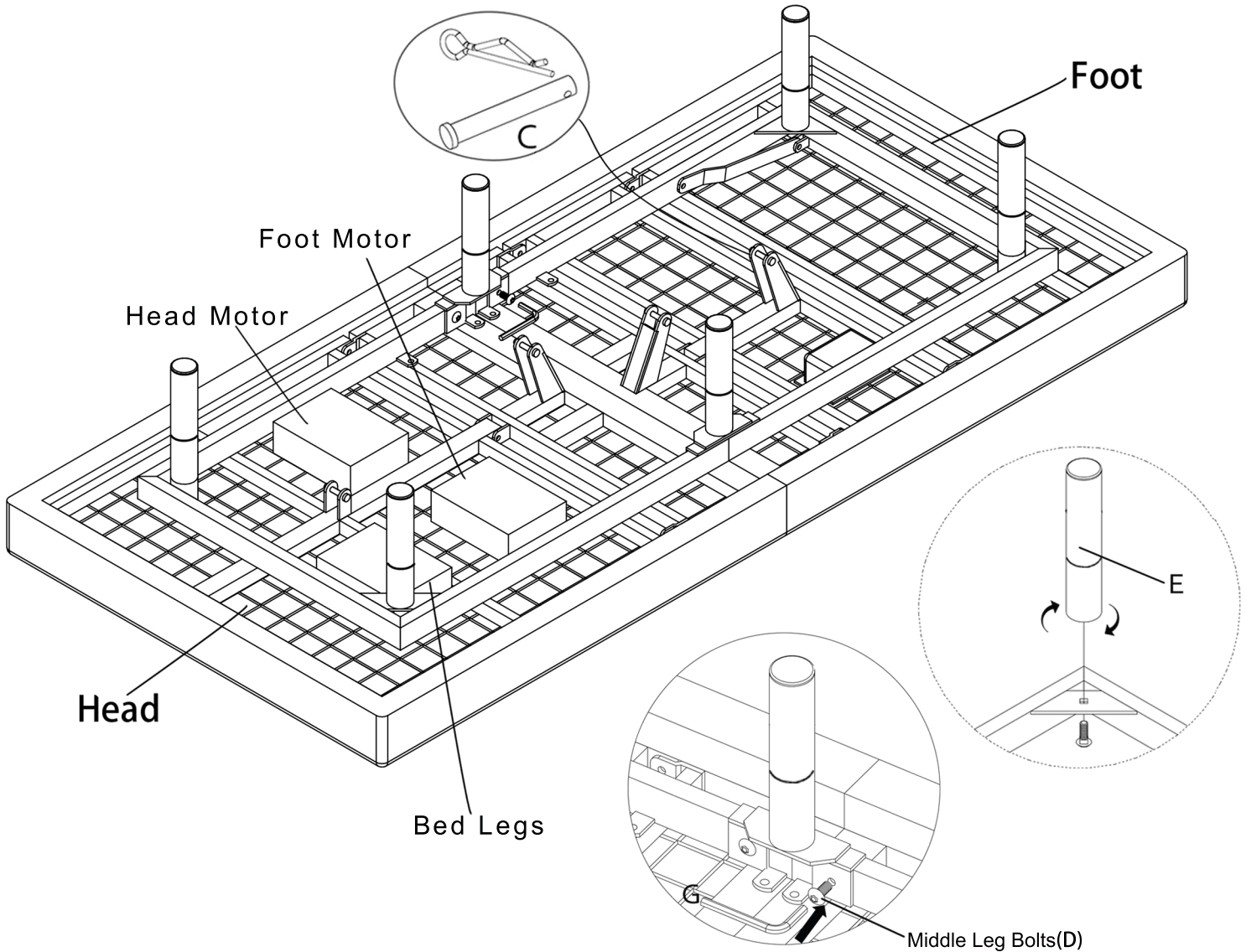
E Corner legs, 4pcs Corner leg bolts, 4pcs
