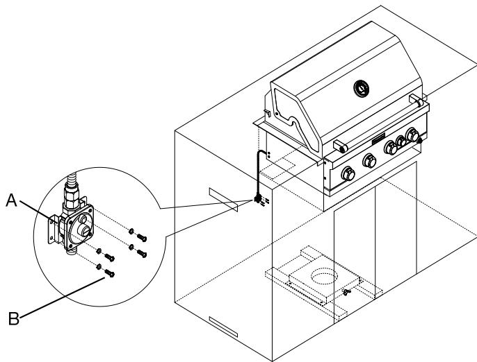
A. Natural gas pressure regulator B. Four 5/32" x 10 mm truss head screws
