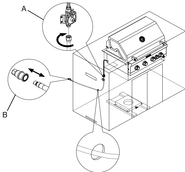
A. Brass connector B. Quick connector
