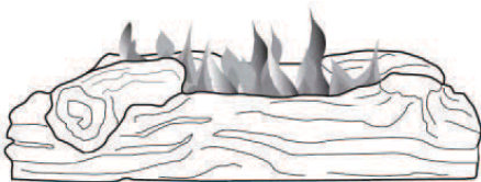
Figure 10 - Correct Burner Flame Pattern
