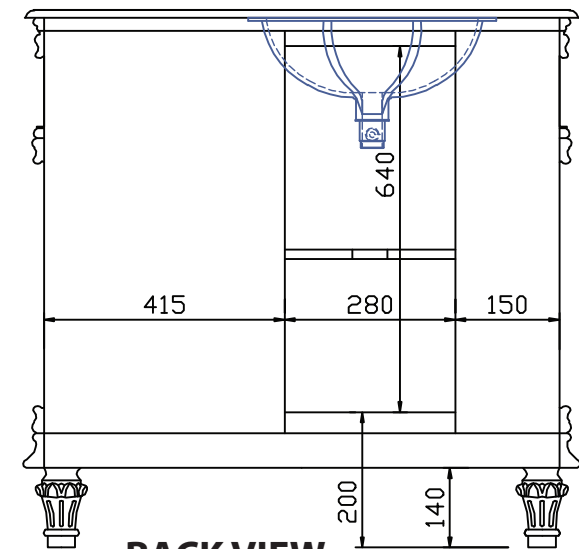
BACK VIEW
