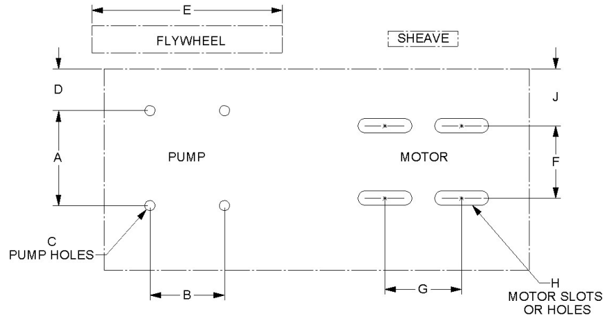
COMPRESSOR PLATFORM LAYOUT
