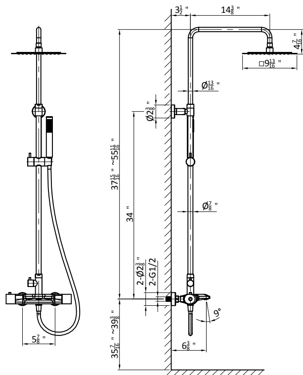
Installation drawing
