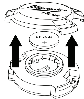
Fig. B REMOVE COVER AND BATTERY
