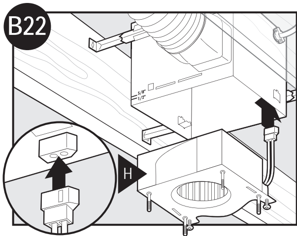
B22 Connect wiring from the motor to the wiring cover plate.
