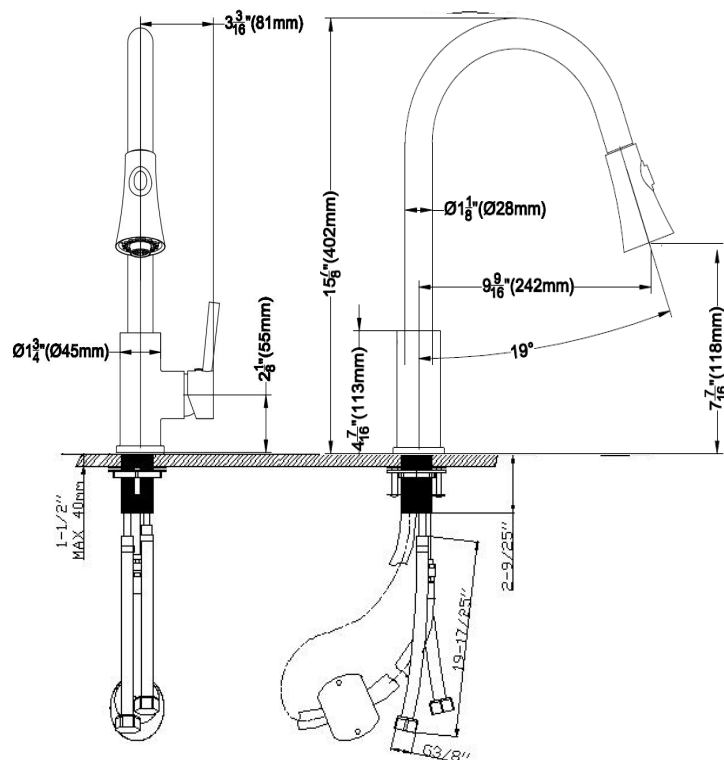
CRITICAL DIMENSIONS
