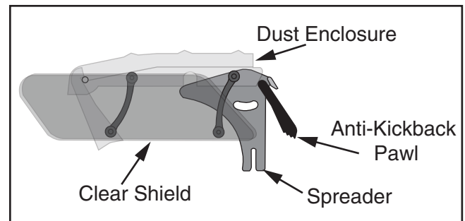
Figure 46. Blade guard assembly components.
