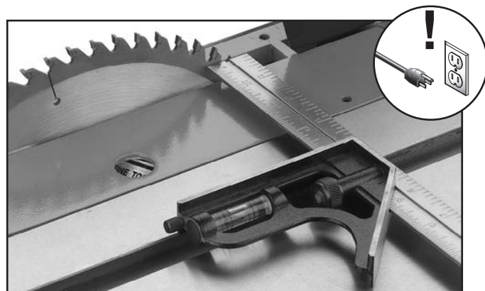
Figure 108. Measuring distance from miter slot to carbide tip on opposite side of table insert.
