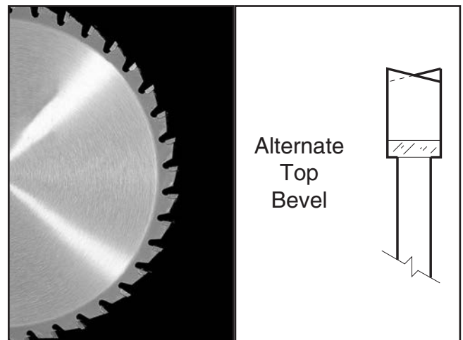
Figure 39. Crosscutting blade.
