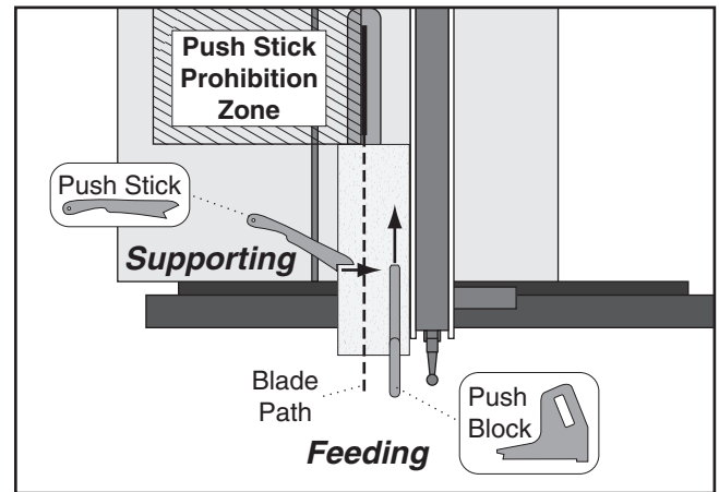
Figure 85. Using a push block and push stick to make a rip cut.
