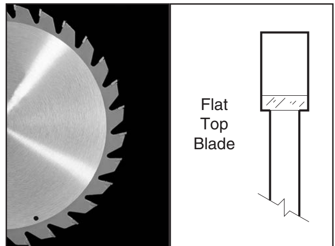
Figure 38. Ripping blade.
