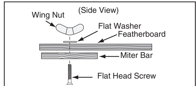
Figure 78. Assembling miter slot featherboard components.
