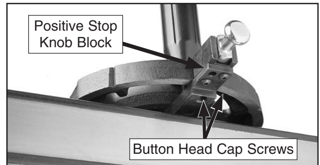
Figure 124. Screws for adjusting miter body.
