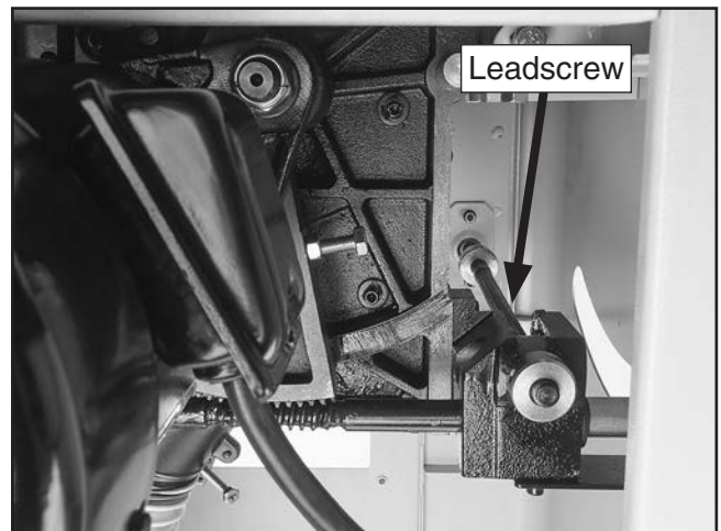
Figure 101. Leadscrew location.
