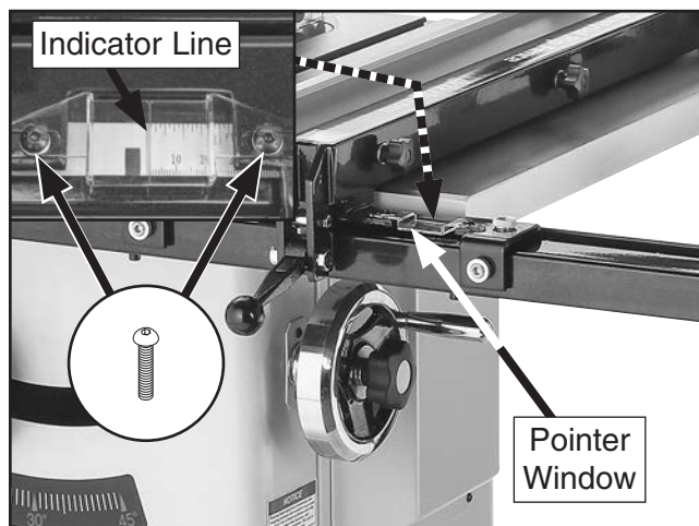
Figure 28. Aligning rail tape with scale pointer.
