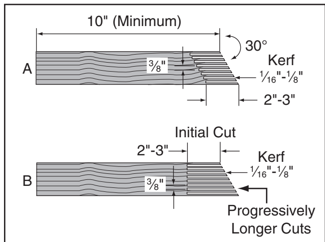
Figure 75. Patterns for featherboards (top view shown).
