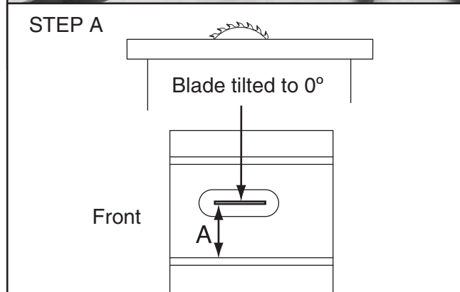
Figure 107. Example of adjusting blade to miter slot.
