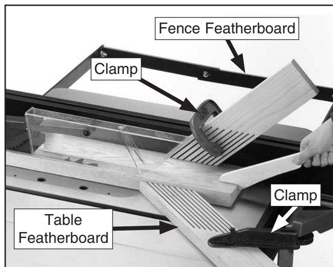
Figure 79. Example of featherboards secured with clamps.
