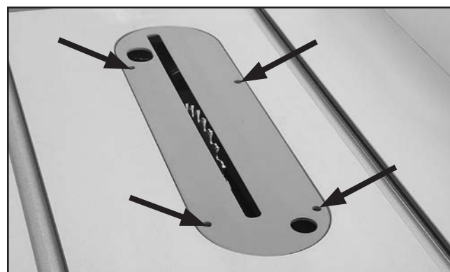
Figure 121. Location of table/dado insert holes with adjustment screws.
