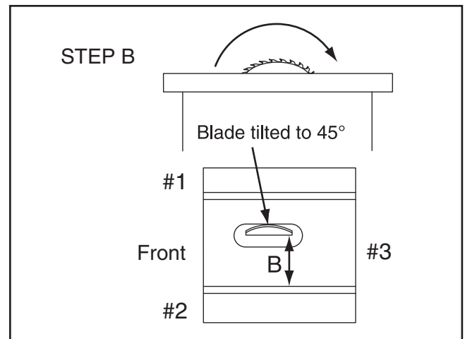
Figure 111. Shim procedure diagram B.
