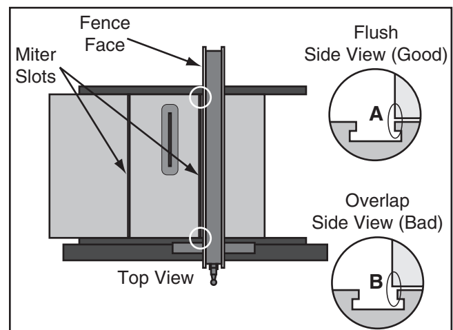
Figure 118. Example of aligning fence to miter slot.
