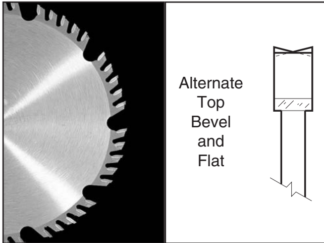
Figure 40. Combination blade.
