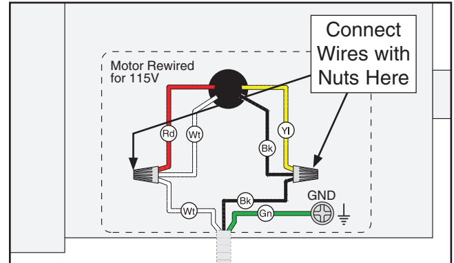
Figure 7. Motor rewired to 115V.
