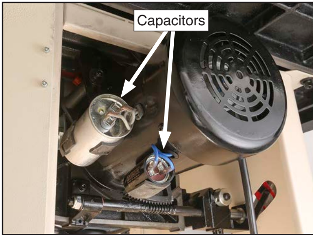
Figure 127. Motor capacitors.
