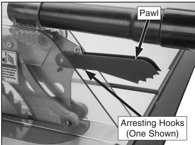
Figure 52. Pawls disabled.
