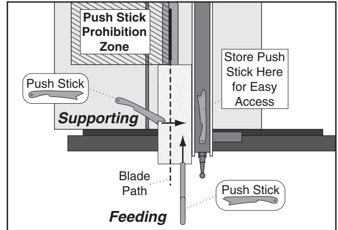
Figure 81. Using push sticks to rip narrow stock.
