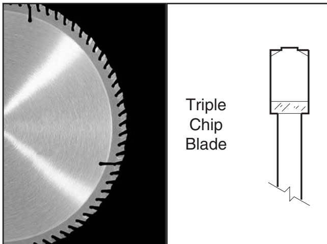
Figure 41. Laminate blade.
