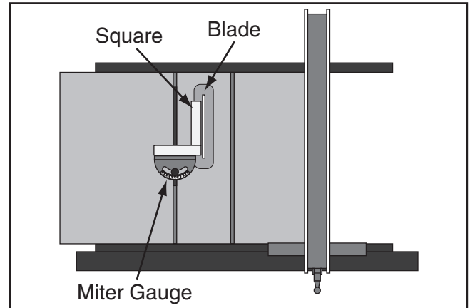
Figure 123. Checking 90° stop on miter gauge.
