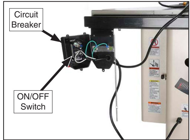
Figure 129. Switch box components.
