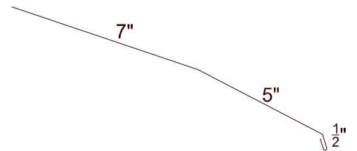
VALLEY RV-1
